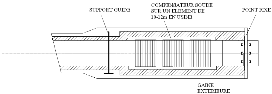
Figure 4 - Compensateur
